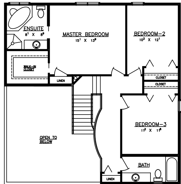
SECOND FLOOR AREA = 882 S.F.
